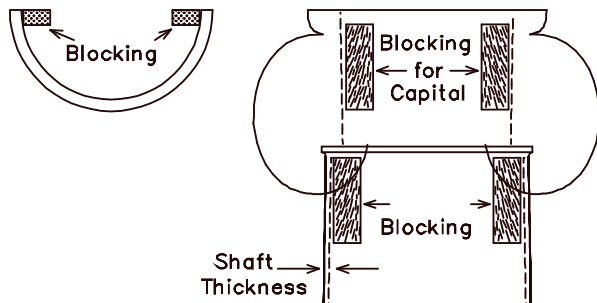
Diagram A – for Ornamental Capitals
