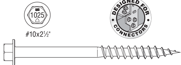
#10 x 2 1/2" Strong-Drive® SD Structural-Connector Screw U.S. Patent 7,101,133
